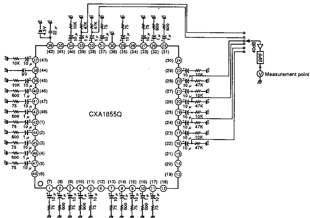
Fig 7. Audio system (residual noise)
